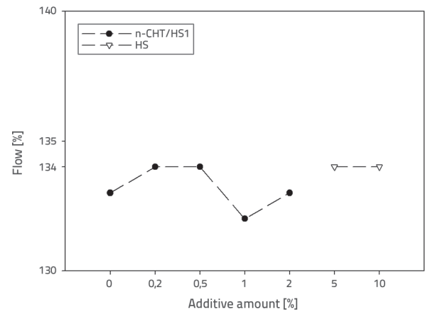
Figure 7. Flowability results
