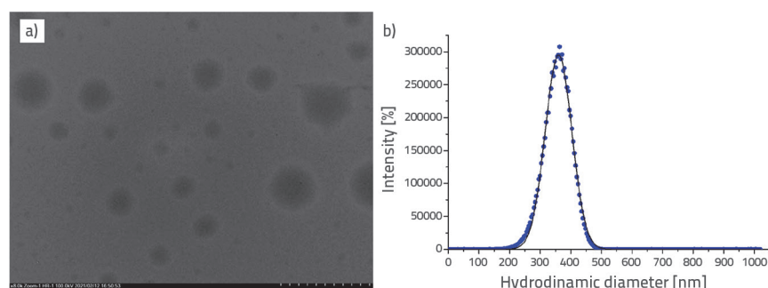
Figure 2. a) TEM micrograph; b) DLS curve of CHT/HS nano-composite
